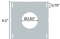
3" Mounting Plate SL3-MP-R-V2
