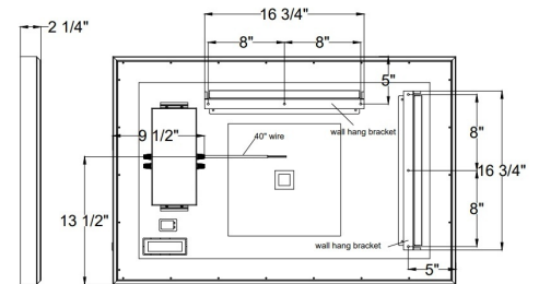
RIGHT SIDE
