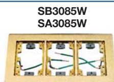
3-Gang Dimensions 6.00" x 11.34"
