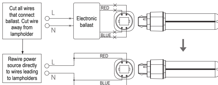
Fig:2 - Electronic ballast fixture wiring
