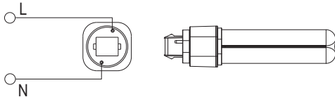
Fig:1 - New fixture without ballast wiring
