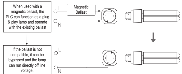
Fig:3 - Magnetic ballast fixture wiring modification
