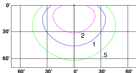
90W 30' Mounting Height 45° tilt
