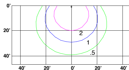
50W 20' Mounting Height 45° tilt
