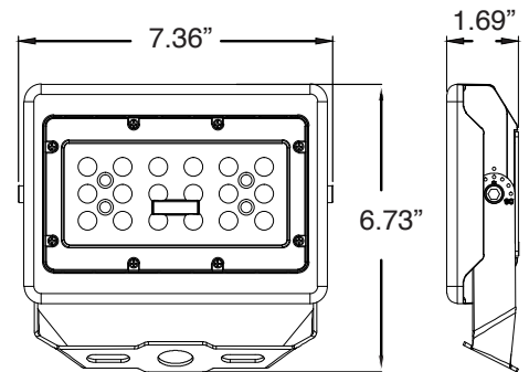
29W with Yoke Mount
