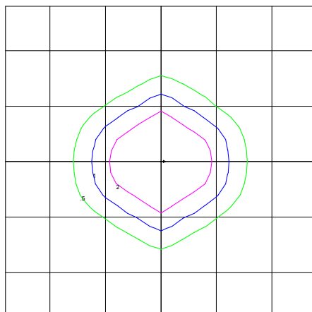
PSM78 25' MTG HT SCALE: 1 INCH = 20 FT.
