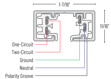
Two-Circuit Track
