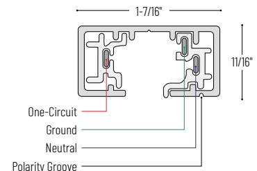
One-Circuit Track
